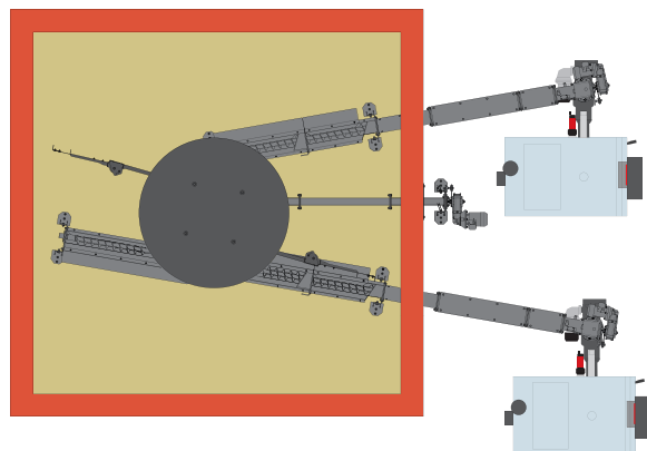
Two discharge screws, one standard, one extra-long
