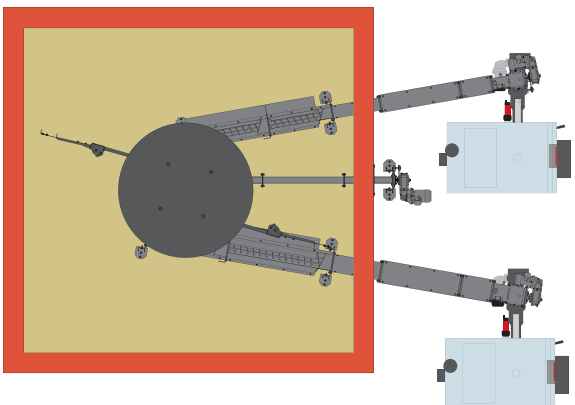
Dual boiler system with two discharge screws
